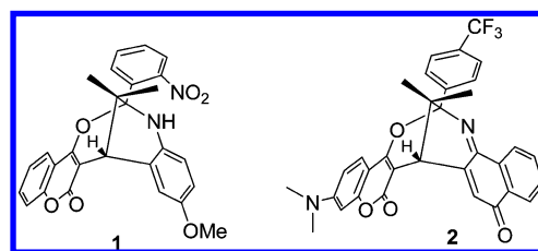
Figure 1. Structures of two oxazabicyclics that possess molecular switching properties screened from MCRs.
